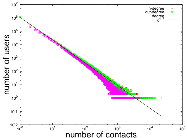
Figure 1: The in-degree and the out-degree distribution measured in the Flickr directed contact network, and the degree distribution measured in the Flickr undirected mutual contact network.
