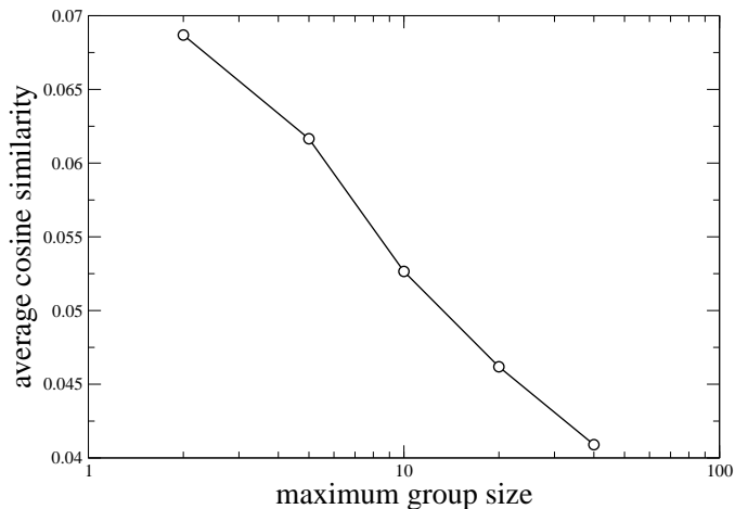
Figure 3: The average tag cloud cosine similarity computed in groups with less than S_{max} members.
