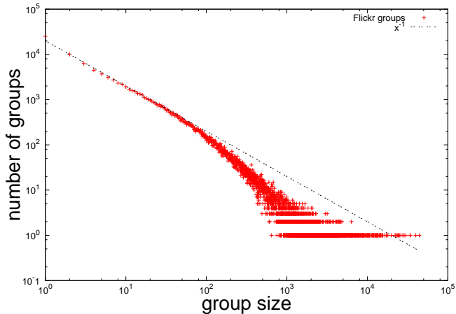
Figure 2: The distribution of the size of Flickr groups.
