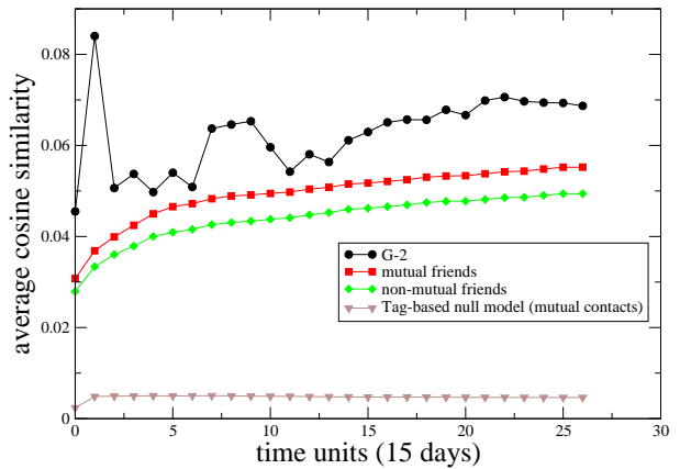
Figure 4: The time evolution of the cumulative cosine similarity for different social networks and the null model.
